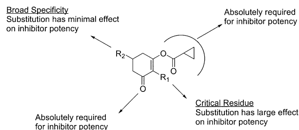
Figure 2. General SAR for 3-cyclopropanecarbonyloxy-2-cyclohexen-1-one inhibitors.
