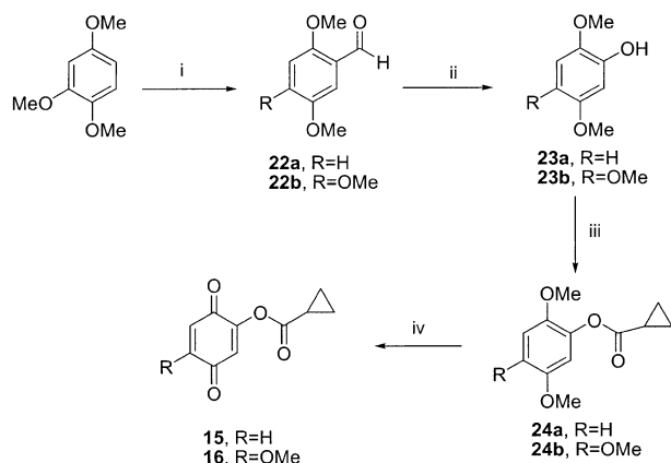
Scheme 3. Preparation of compounds 15 and 16 : (i) POCl 3 , DMF; (ii) H 2 O 2 , H 2 SO 4 , MeOH; (iii) cyclopropanecarbonyl chloride, Et 3 N, CH 2 Cl 2 ; (iv) Ag 2 O, 6 N HNO 3 , acetone.
