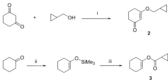
Scheme 1. Synthesis of compounds 2 and 3 : (i) p -TsOH, benzene, reflux; (ii) Et 3 N, trimethylsilyl chloride, DMF, 120 °C; (iii) potassium t -butoxide, cyclopropanecarbonyl chloride, THF, –20 °C.
