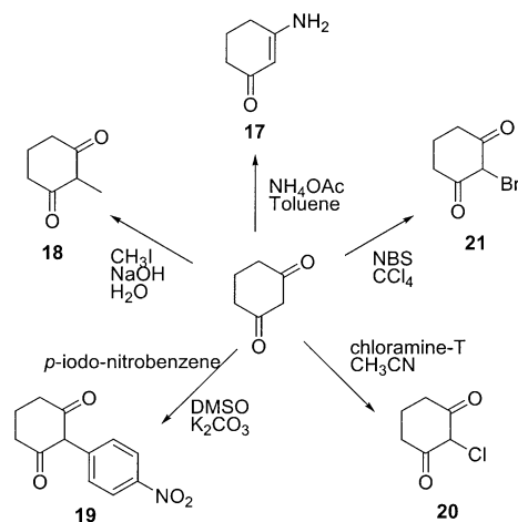
Scheme 2. Preparation of compounds 17–21 .
