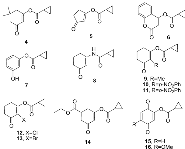
Figure 1. Various compounds synthesized for SAR studies.
